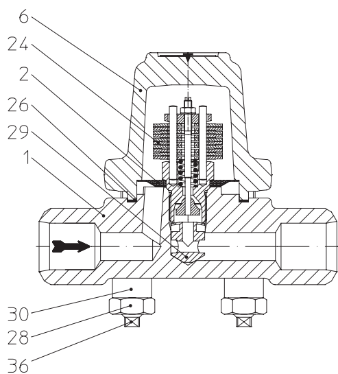
Рис. 6: CONA®B - BR600 PN63/100 DN15-25
